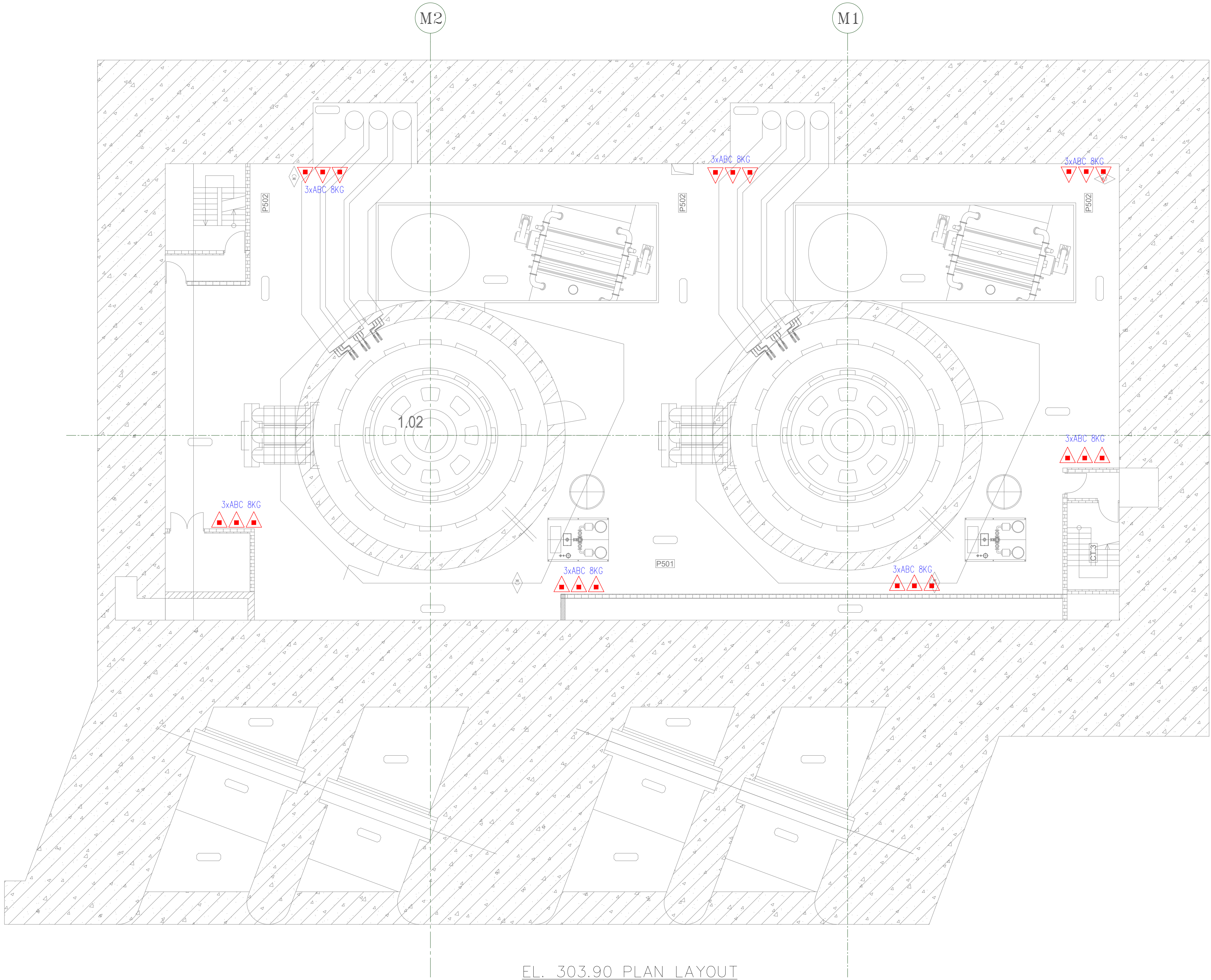
EL. 303.90 PLAN LAYOUT
