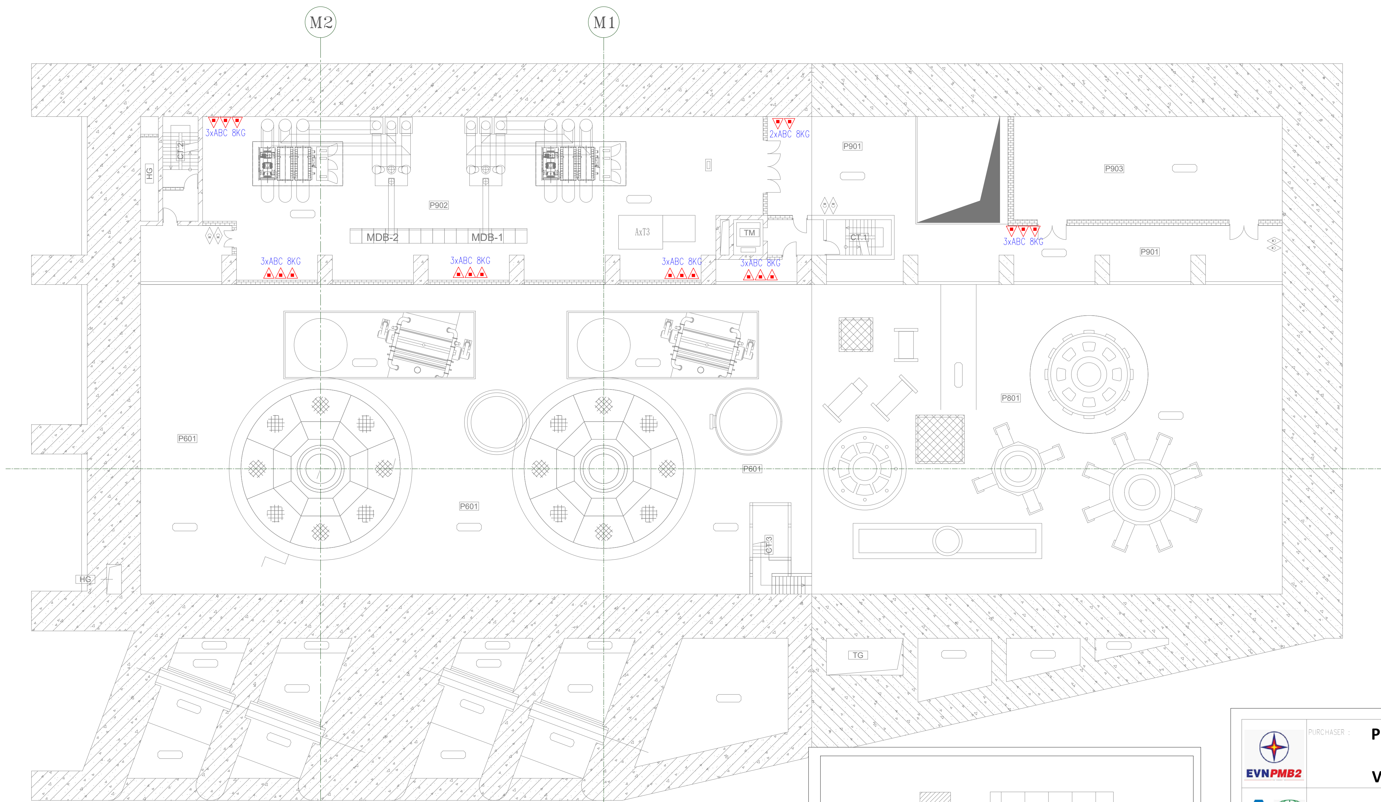
EL. 331.40 PLAN LAYOUT
